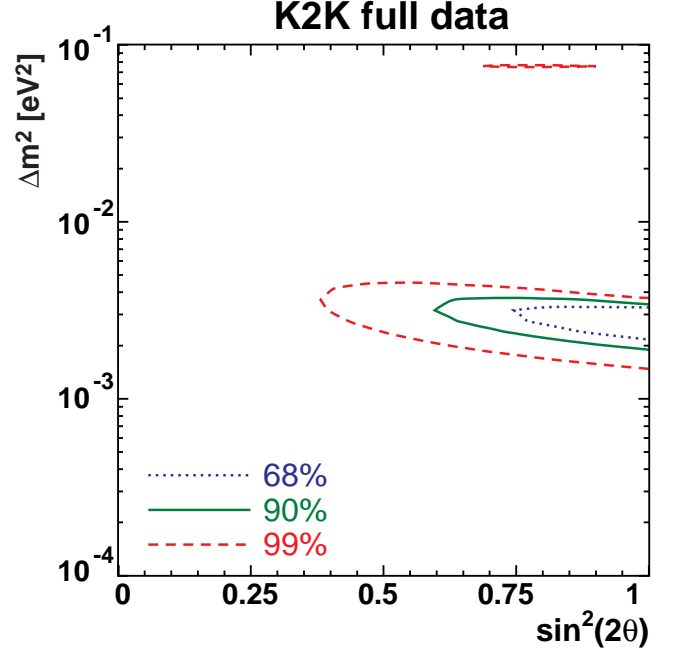
FIG. 44: Allowed regions of oscillation parameters. Three contours correspond to the 68% (dotted line), 90% (solid line) and 99% (dashed line) CL. allowed regions, respectively.
