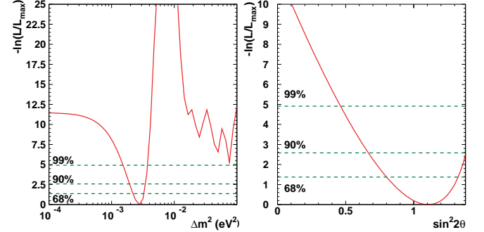
FIG. 45: \ln \mathcal{L}_{\max}^{\text{phys}} - \ln \mathcal{L}(\Delta m^2, \sin^2 2\theta) distribution as a function of \Delta m^2 (left) and \sin^2 2\theta (right). \sin^2 2\theta is set to be 1.0 in the left-hand figure and \Delta m^2 is set to be 2.8 \times 10^{-3} eV 2 in the right-hand figure. Three horizontal lines correspond to the 68%, 90% and 99% CL interval from the bottom one, respectively.
